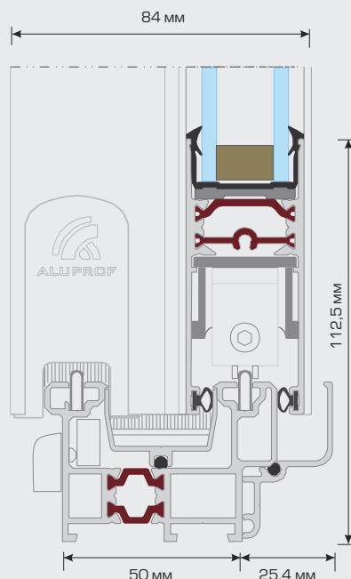
MB-Slide ST
